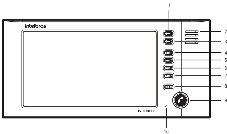
Vista frontal
