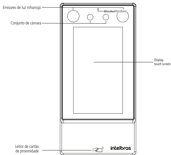
Vista frontal SS 3532 MF
