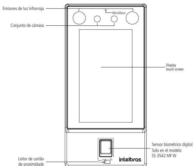
Vista frontal SS 3542 MF W
