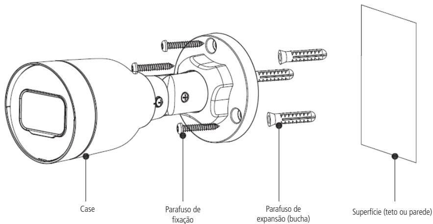
Vista detalhada VIP 1130 B G4, VIP 1230 B G4, VIP 1230 B Black G4 e VIP 1220 B Full Color G4
