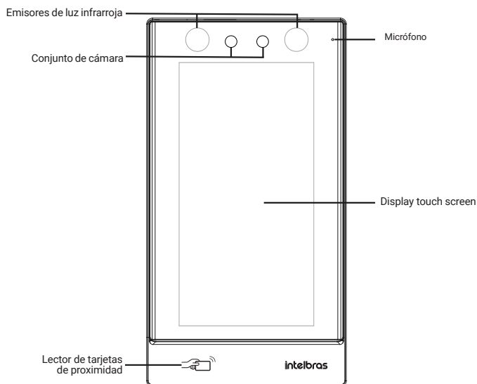
Vista frontal SS 5531 MF W
