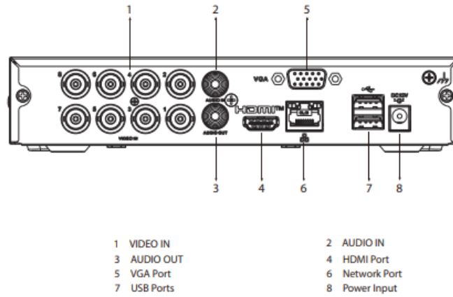
Figura 1 - Painel MHDX 1108-C
