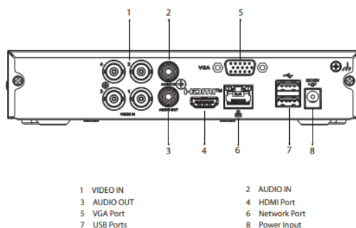
Figura 1 - Painel MHDX 1104-C
