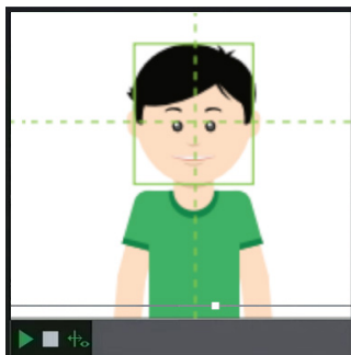
Playback
