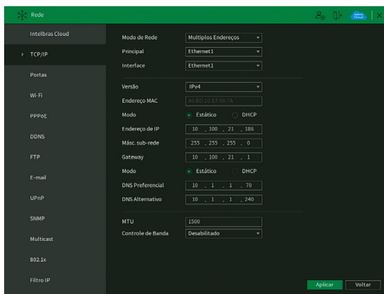
Menu TCP/IP
