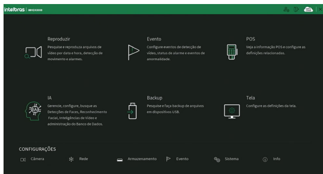
Menu Principal
