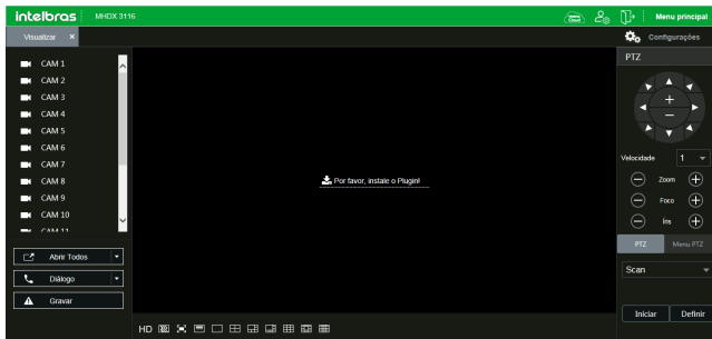
Tela principal
