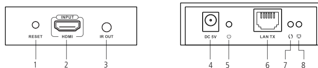
Transmissor
