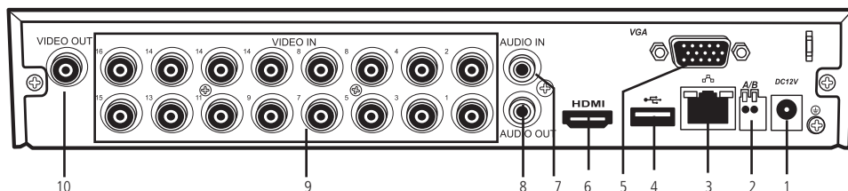
Painel traseiro
