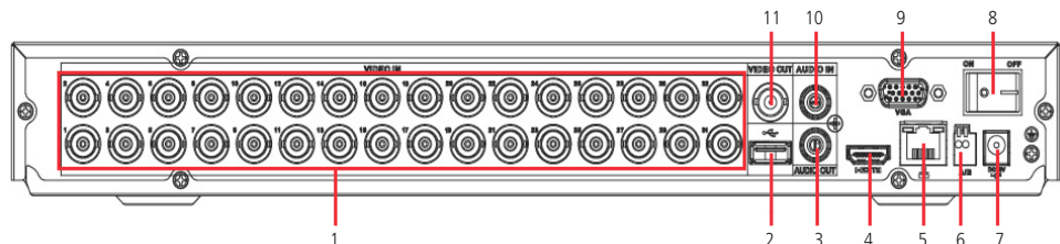
Painel traseiro
