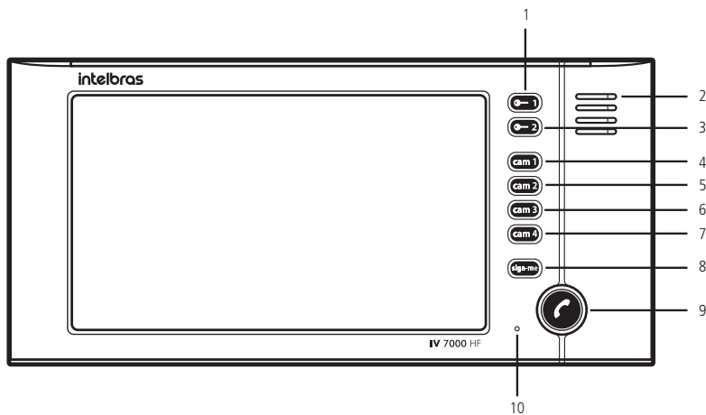
Vista frontal
