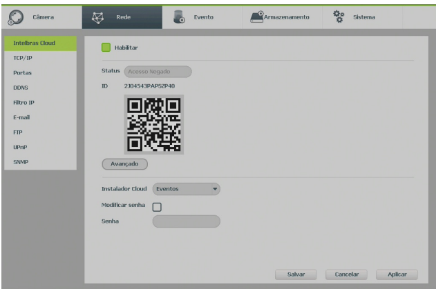
Intelbras Cloud
