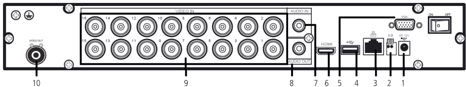
Painel traseiro
